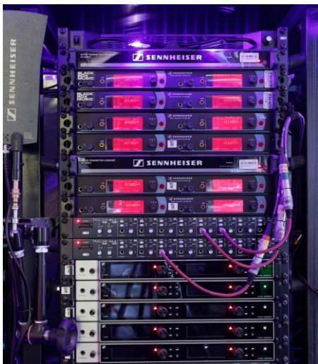
2000 series IEM transmitters and Digital 6000 microphone receivers from Sennheiser
